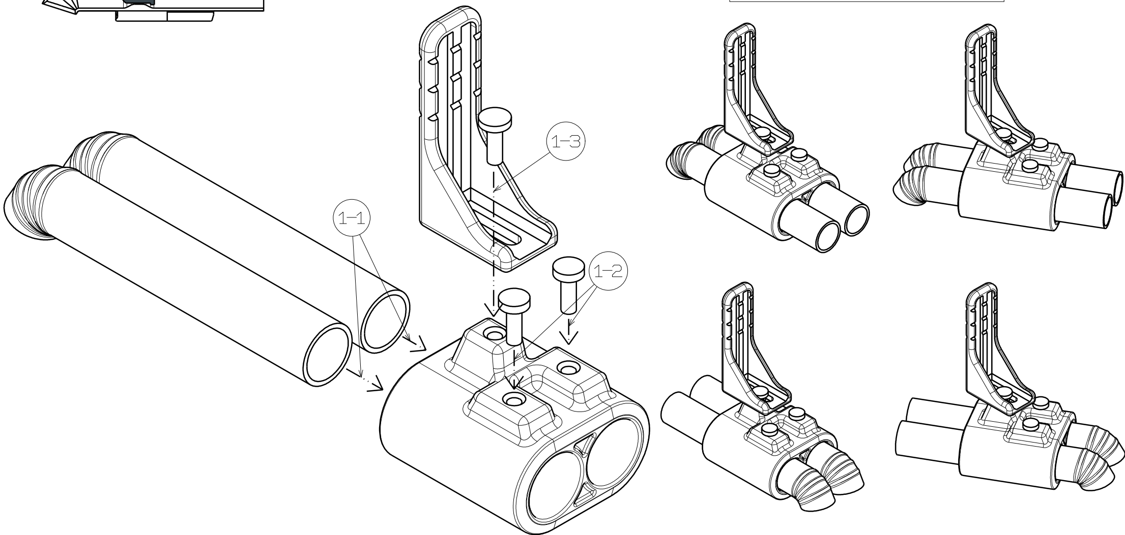
完成図(Completion drawing)
